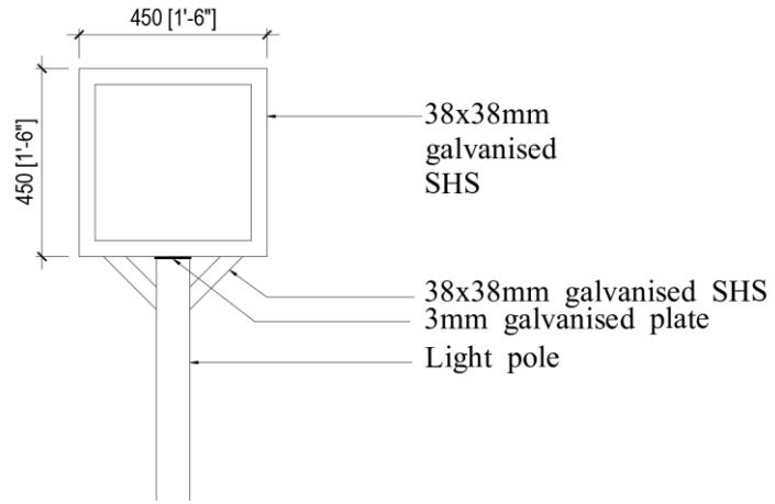
Figure 3: Light pole top section
