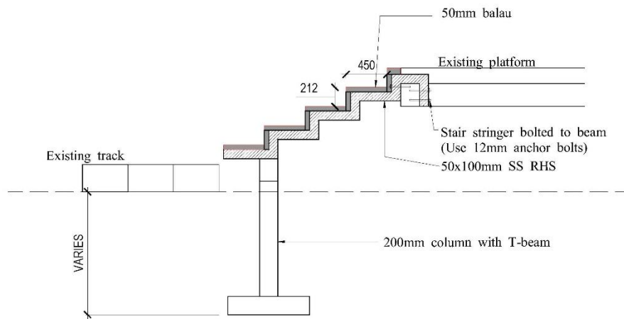
STAIR-SECTION
